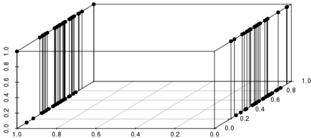
Figure 27: Two binary variable and one continuous variable
