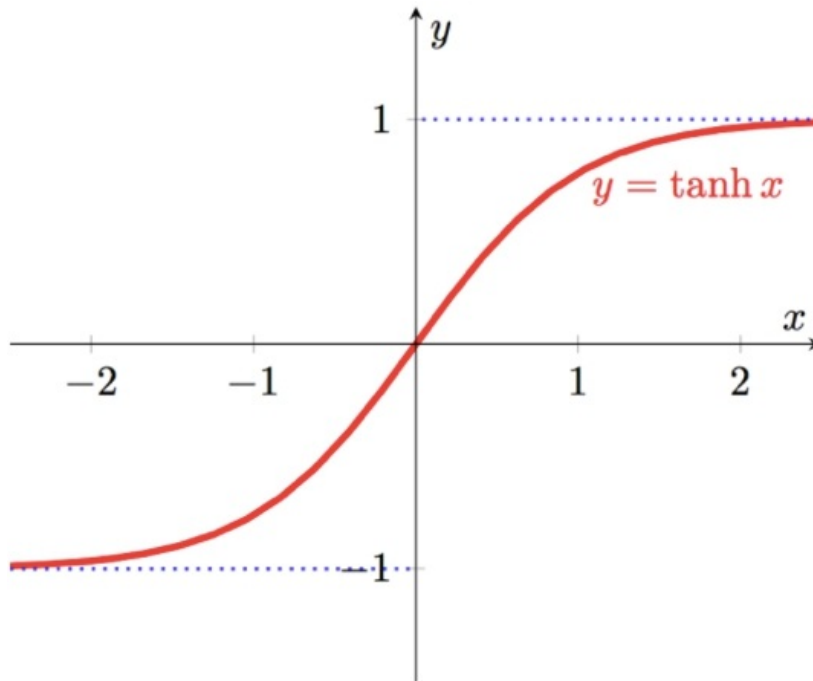
Figure 52: A hyperbolic tangent function graph
