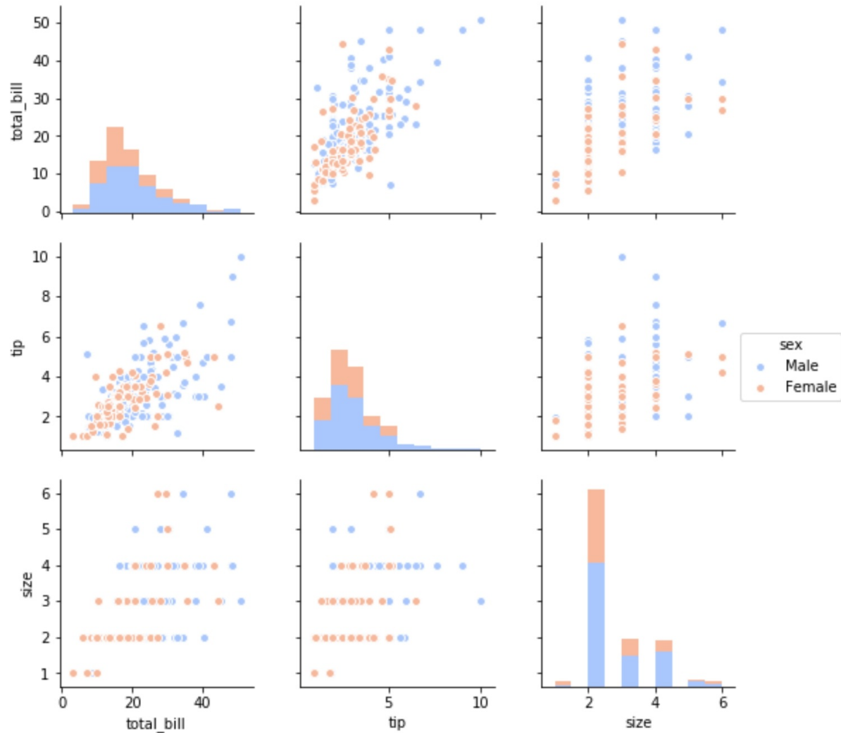
Figure 20: Pairplot with three variables
