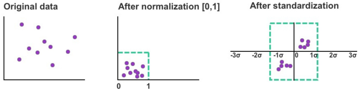
Figure 10: Examples of rescaled data using normalization and standardization
