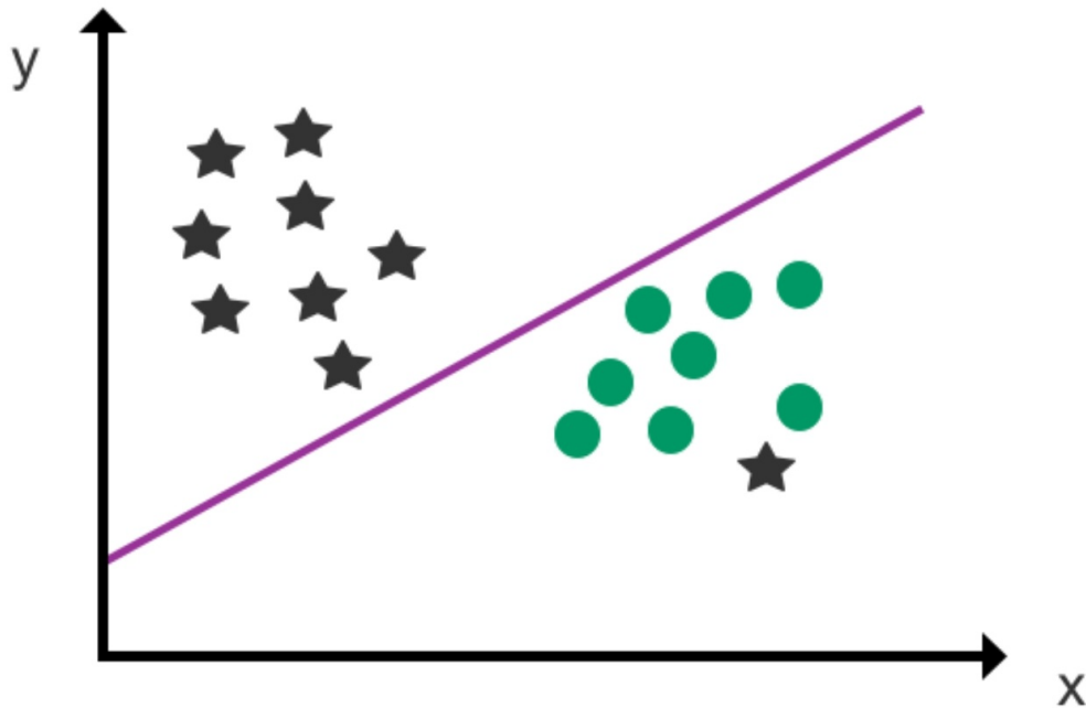
Figure 23: An example of logistic regression
