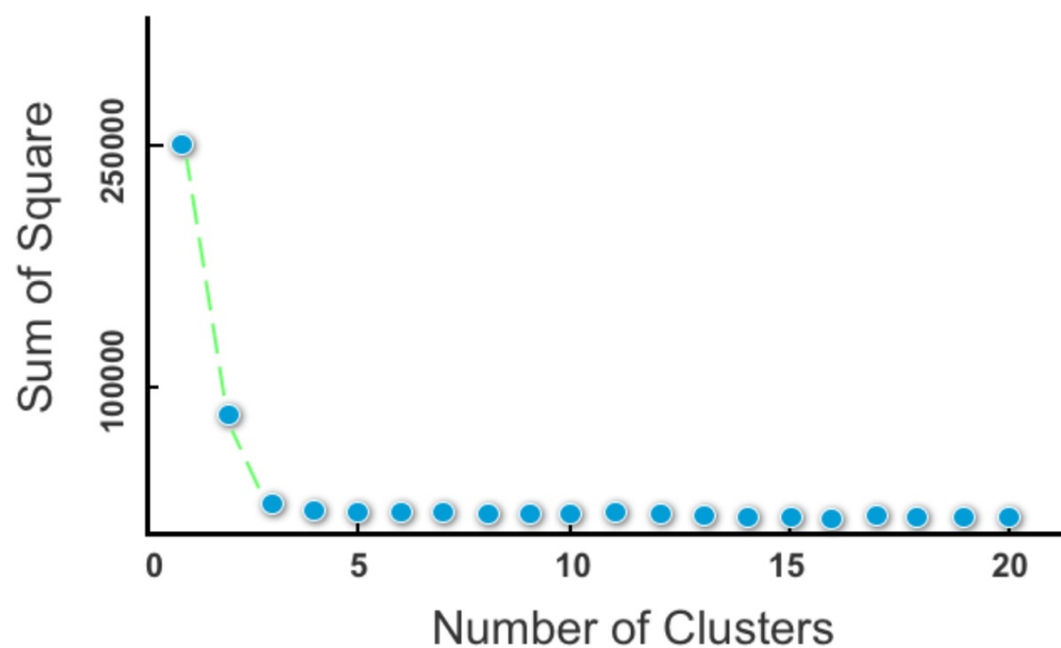
Figure 35: A scree plot
