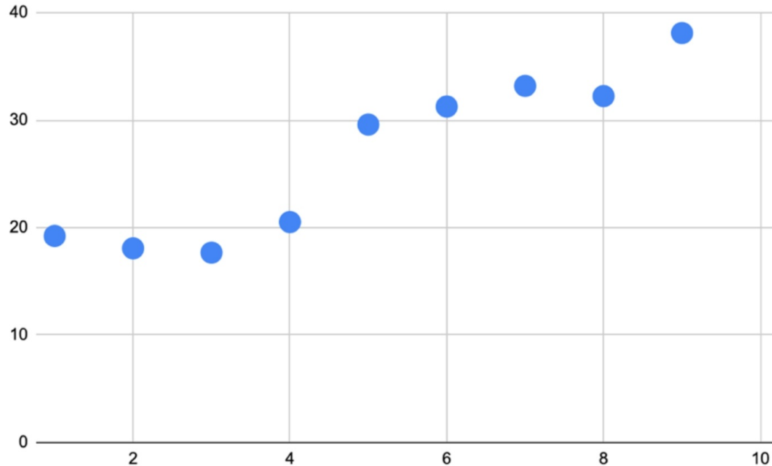
Figure 14: Seinfeld dataset plotted on a scatterplot
