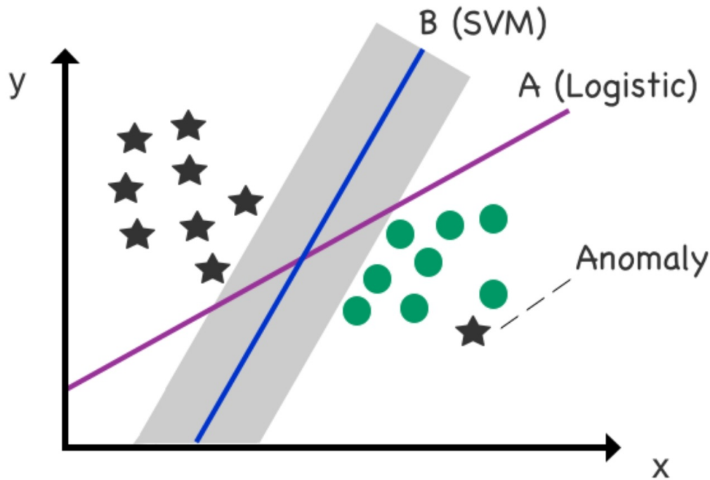
Figure 42: Mitigating anomalies
