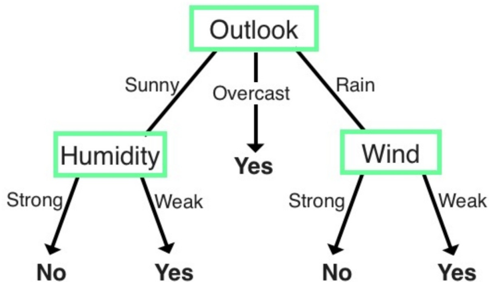
Figure 56: Example of a classification tree
