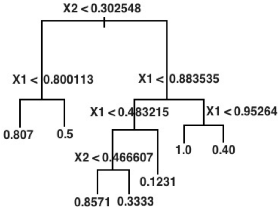
Figure 55: Example of a regression tree
