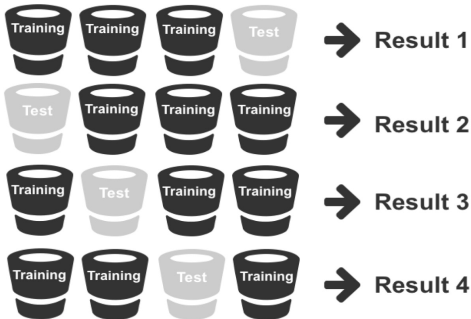
Figure 13: k -fold validation
