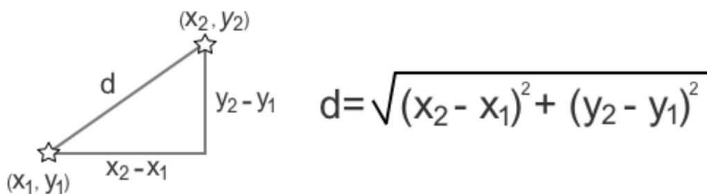
Figure 29: Calculating Euclidean distance
