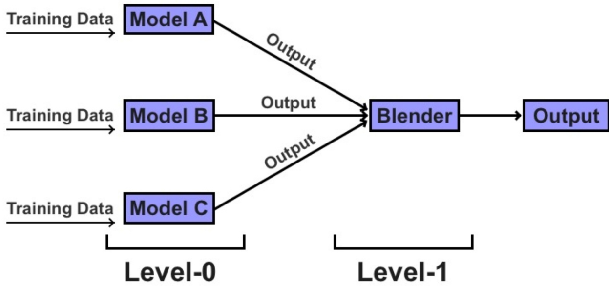
Figure 59: Stacking algorithm
